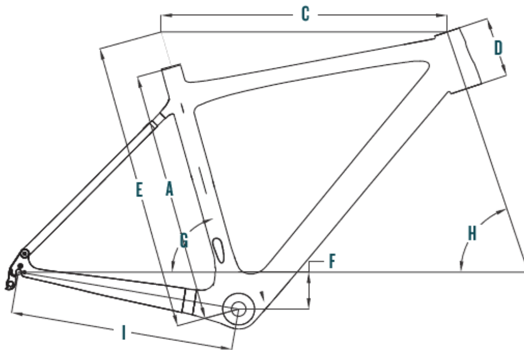
CLEMENTINE 916 GEOMETRY CHART
